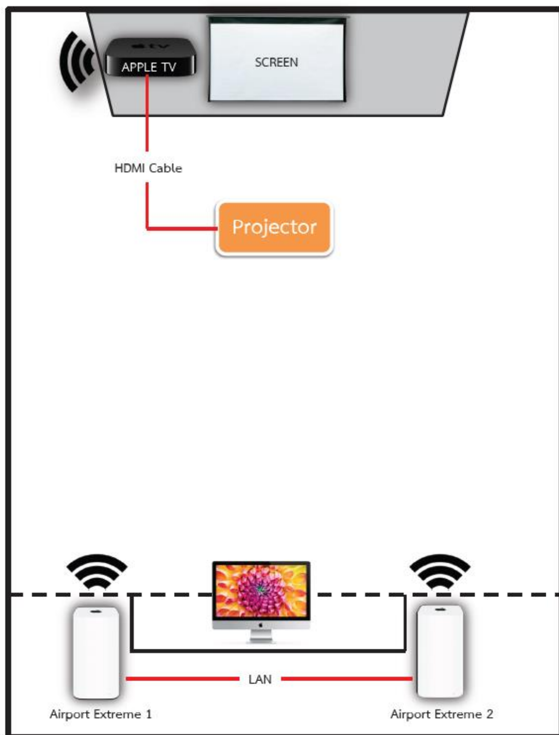
iClassroom Kanlayanawat System Diagram
